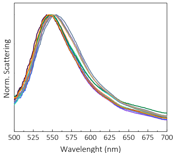
Figure S4. Normalized scattering spectra of 12 different Au NPs used as seeds, where the different maximums account for the size distribution.
