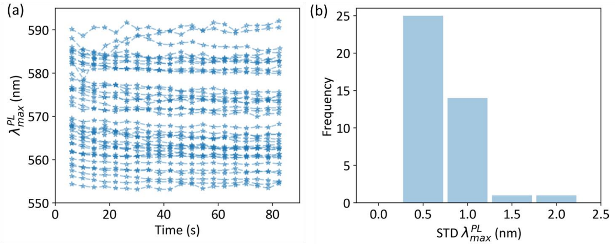
Figure S2. (a) \lambda_{max}^{PL} (nm) vs. time for 41 different Au NPs measured during 80 s on water with a laser irradiance of 2.6 \text{ mW} \cdot \mu\text{m}^{-2} . The PL was measured for Au NPs with a \lambda_{max}^{PL} (nm) > 550 nm. (b) Histogram of the standard deviation of \lambda_{max}^{PL} on time ( \text{STD } \lambda_{max}^{PL} (nm)) for 41 Au NPs. The mean value of \text{STD } \lambda_{max}^{PL} was 1 nm.
