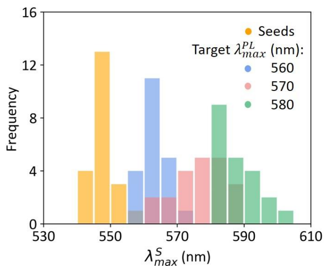
Figure S5. Histogram of \lambda_{max}^S of 21 different Au NPs before plasmon-driven growth (seeds) and grown to three different \lambda_{max}^{PL} targets: 560, 570 and 580 nm. The means and standard deviations of the \lambda_{max}^S distributions are: (547 \pm 3) nm for the seeds, (563 \pm 4) nm for the NPs with target \lambda_{max}^{PL} of 560 nm, (576 \pm 7) nm for the NPs with target \lambda_{max}^{PL} of 570 nm, and (588 \pm 7) nm for the NPs with target \lambda_{max}^{PL} of 580 nm.
