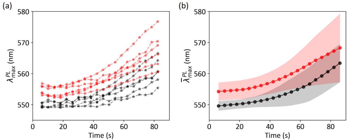
Figure S3. (a) Maximum of PL emission \lambda_{max}^{PL} vs. time for 12 Au NPs grown during 80 s under identical conditions: irradiance = 2.6 \text{ mW} \cdot \mu\text{m}^{-2} , 0.5 \mu\text{M} \text{HAuCl}_4 . Black color corresponds to 6 NPs with 549 \text{ nm} < \text{initial } \lambda_{max}^{PL} < 551 \text{ nm} . Red color corresponds to 6 NPs with 553 < \text{initial } \lambda_{max}^{PL} < 557 \text{ nm} . (b) Mean \bar{\lambda}_{max}^{PL} vs. time during plasmon-driven growth. Each color curve corresponds to the average kinetics and shaded areas indicate \pm 2 standard deviations. Black curve has an initial standard deviation of 0.8 nm and final of 3.1 nm. Red curve has an initial standard deviation of 1.5 nm and final of 5.5 nm.
